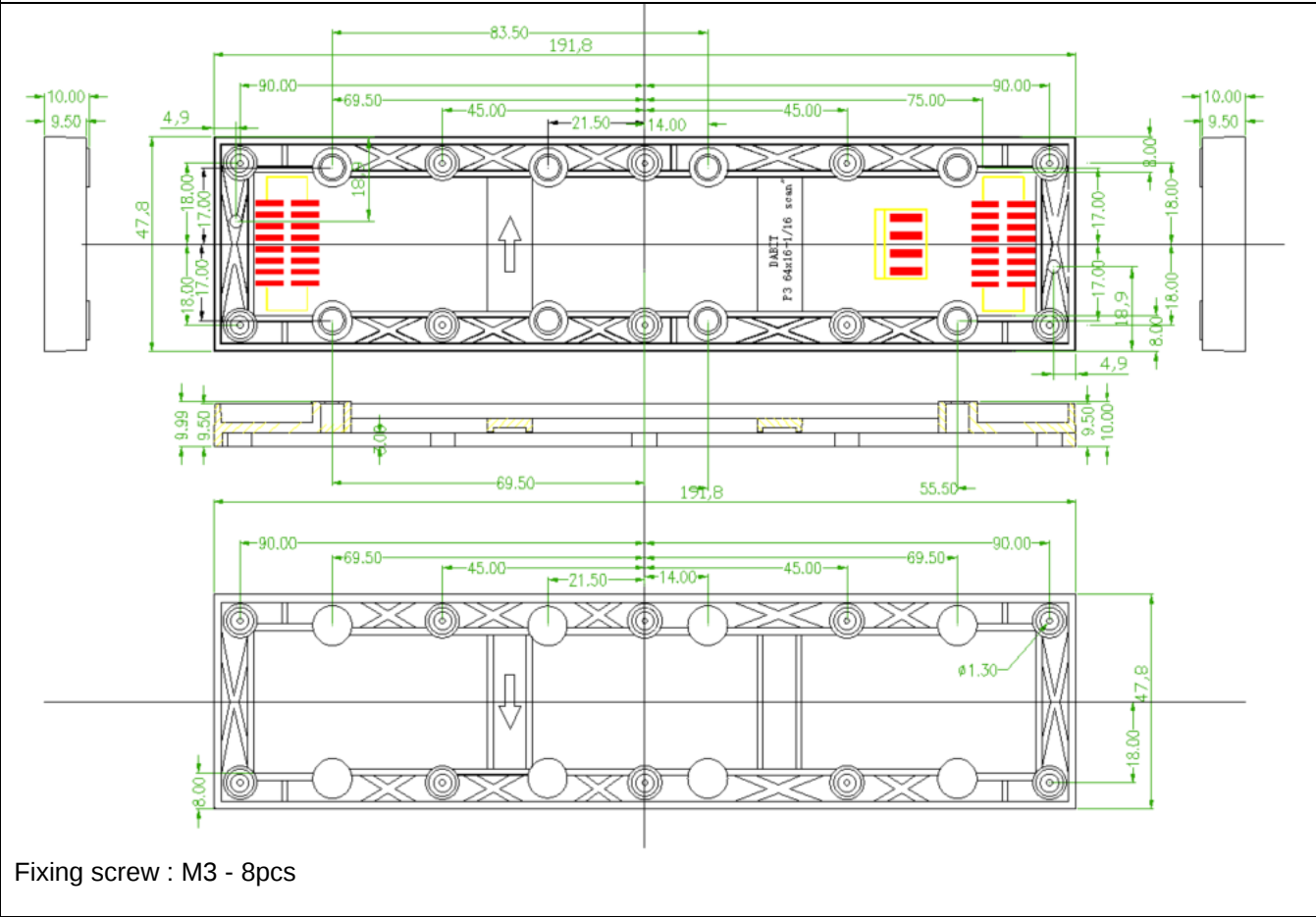
( 5 ) Drawing of the frame
